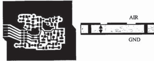
Figure 4. Interconnection layout and dielectric substrate.
