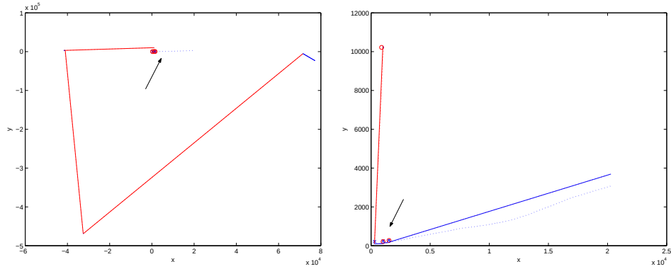
(a) Estimated trajectory using EKF. Estimated trajectory far from true trajectory.
