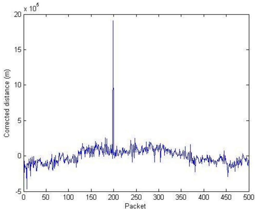
Figure 30: Normalized data to correct for clock drift to be made nearly constant
