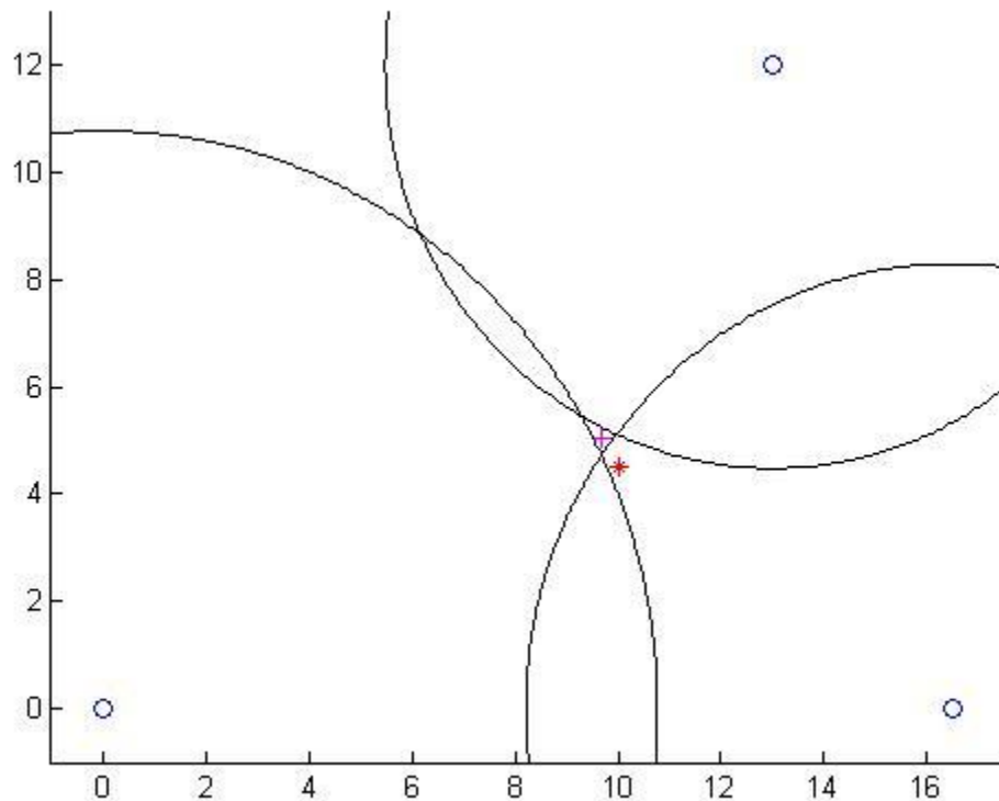
Figure 31: Localization test results showing sensor location and known and estimated transmitter locations
