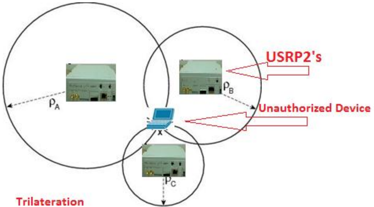
Figure 1: Localization system setup with three USRP2 sensors and a transmitter
