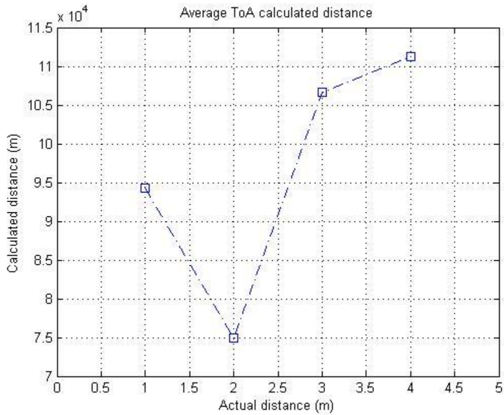
Figure 23: Raw distance results
