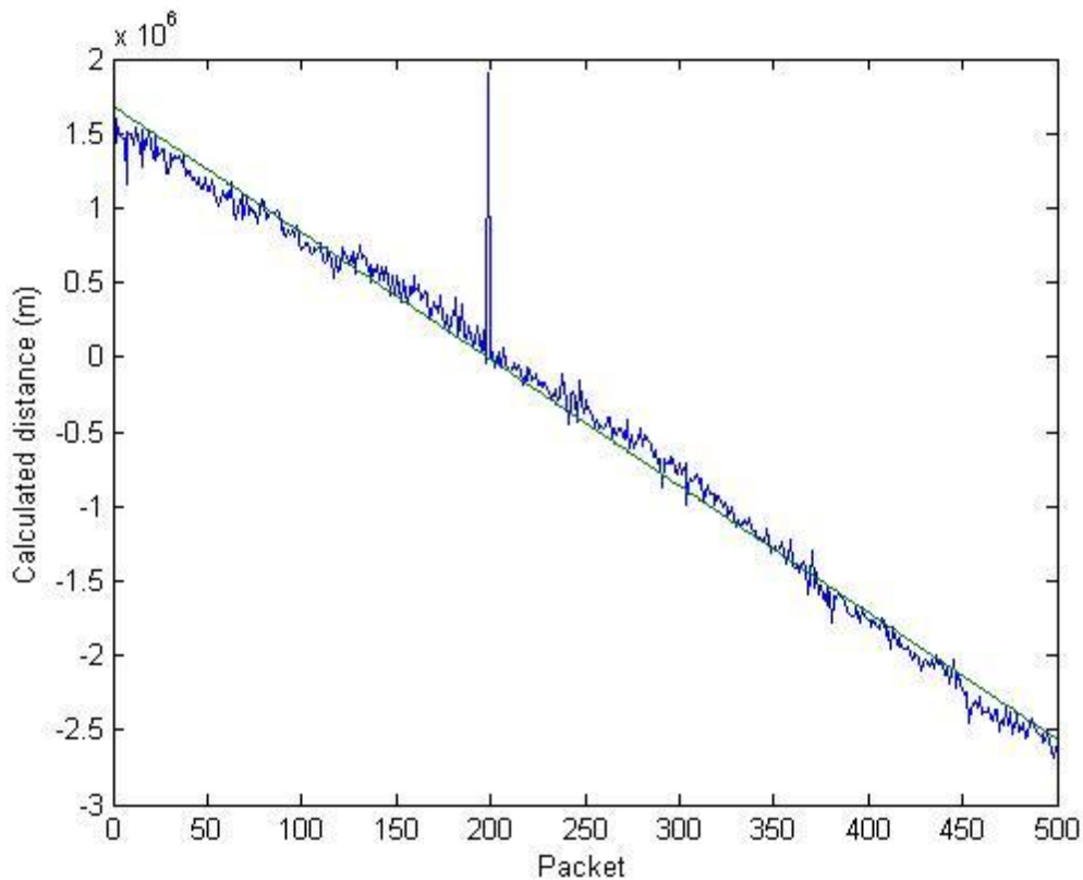
Figure 29: The raw data with best-fit line, clearly showing clock drift
