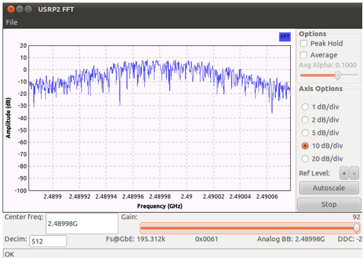
Figure 20: FFT showing effect of too much gain
