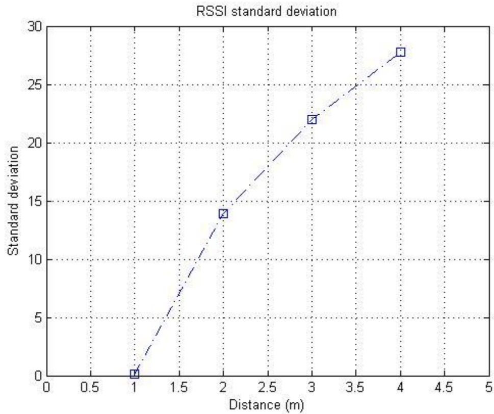
Figure 25: RSSI standard deviation
