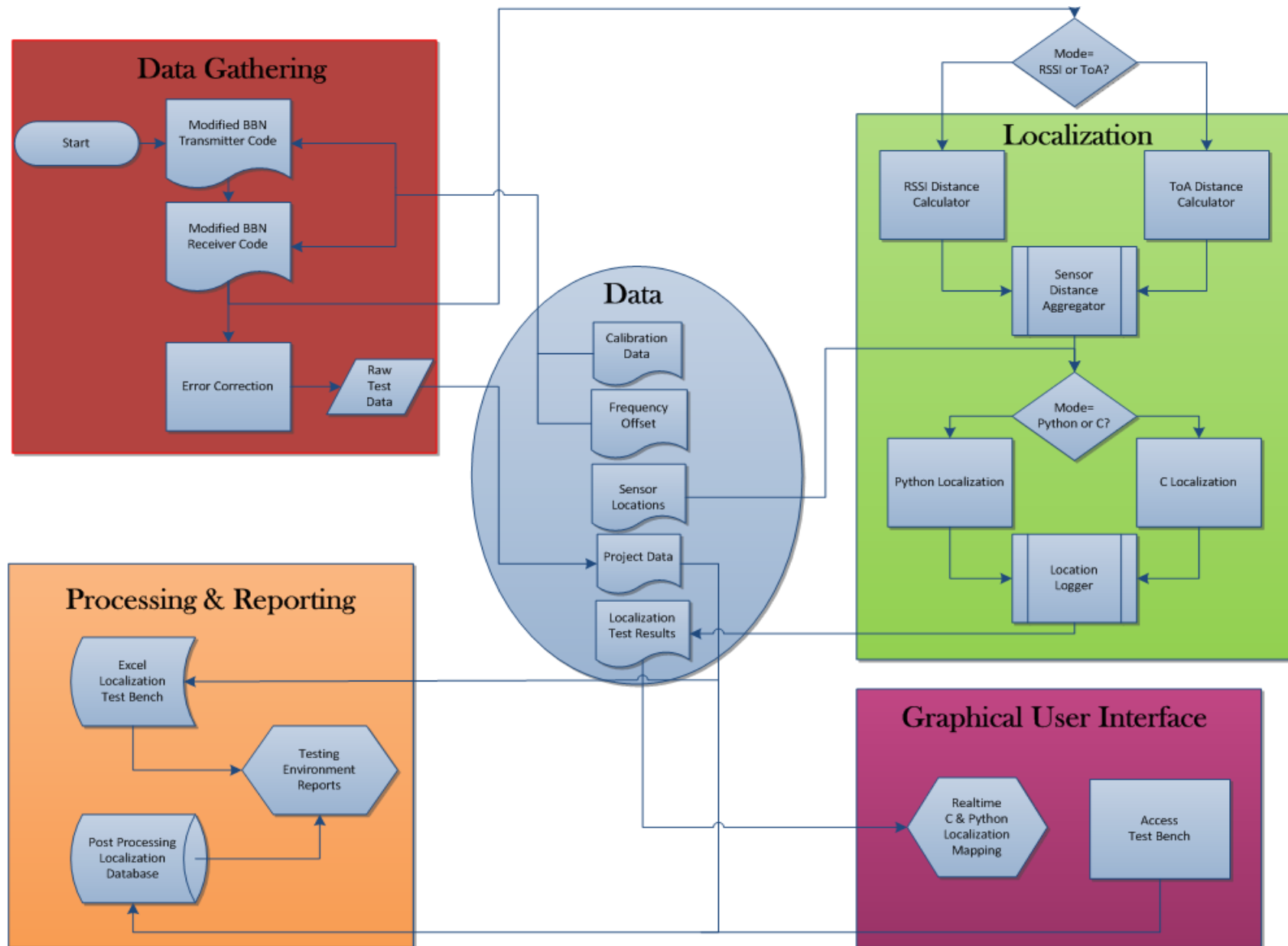
Figure 9: System functionality diagram
