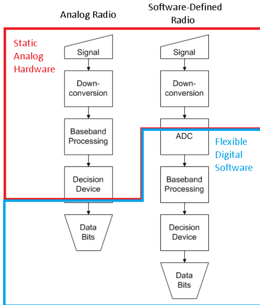
Figure 4: Diagram comparing SDR with analog radio [13]
