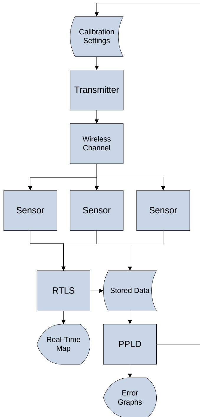
Figure 7: Full system architectural flow graph
