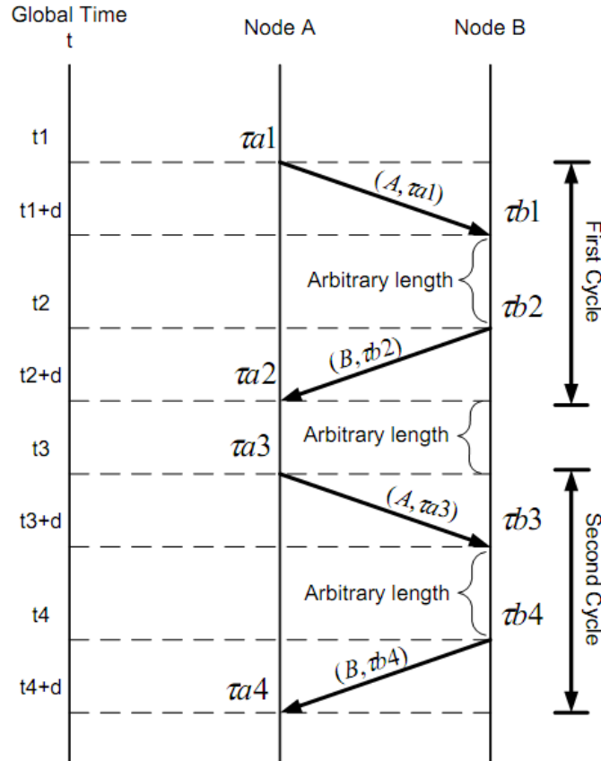
Figure 3: PinPoint DTDOA scheme [11].
