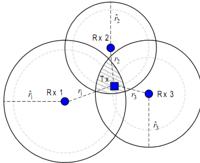
Figure 6: How Range Error Affects Triangulation [31]
