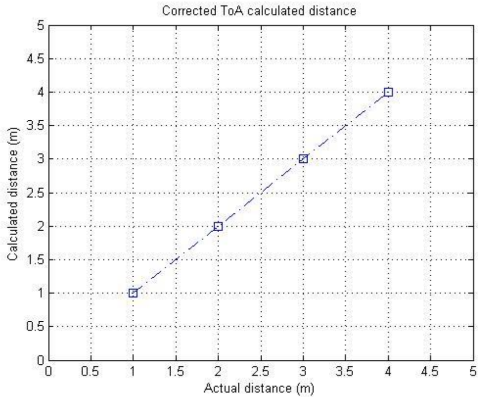
Figure 24: Corrected distance results
