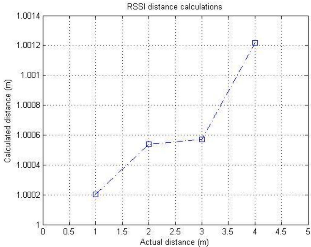
Figure 26: Raw RSSI distance results
