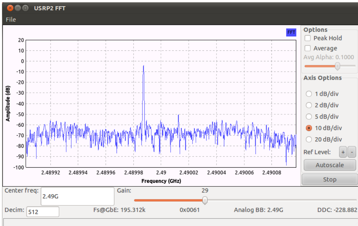
Figure 19: FFT for frequency offset detection
