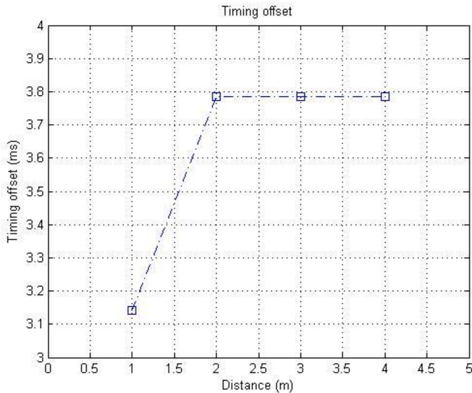
Figure 22: Average timing offsets from data
