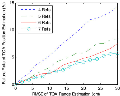
Fig. 8. Failure rate by using TOA based AML method with different number of reference nodes and 500 times' average in a 10\text{m} \times 10\text{m} \times 10\text{m} 3D space.
