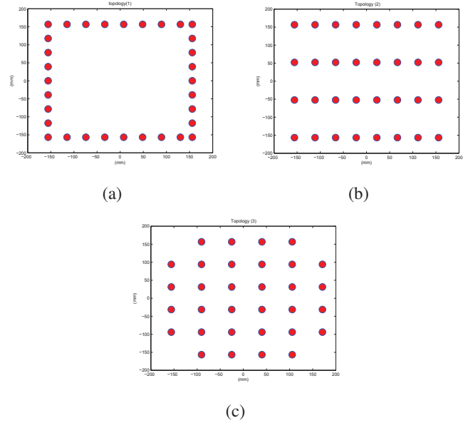
Fig. 8: Three patterns for sensor configuration considered for analysis of the bounds (a)Topology1: square configuration (b)Topology2: parallel line configuration (c)Topology3: grid configuration
