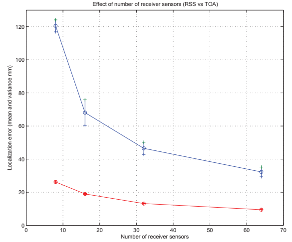
Fig. 7: Performances of RSS- and TOA-based localization as a function of number of receiver sensors.
