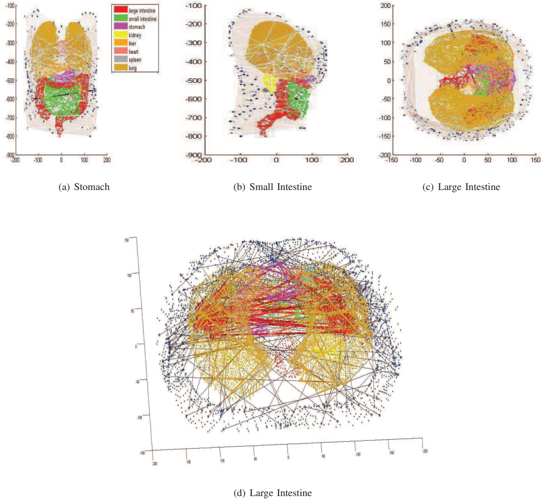
Fig. 4: Simulation scenario for the DME in TOA ranging. The transmitter and receiver pairs are randomly distributed on the surface of body torso. The path length through each organ are marked as different colors in order to calculate the DME caused by tissue non-homogeneity.
