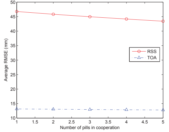
Fig. 11: Performances as a function of number of pills in cooperation for RSS and TOA-based localization
