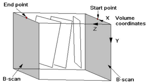
Fig. 5. The construction of the volume coordinates system.
