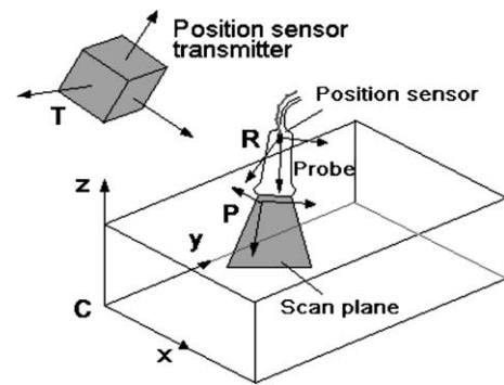
Fig. 1. Coordinate systems in freehand 3D ultrasound imaging system with a position sensor.
