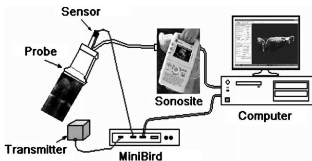
Fig. 2. Diagram of the portable 3D freehand ultrasound imaging system.
