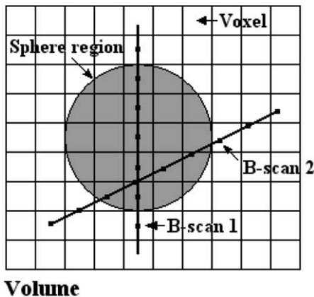
Fig. 7. A 2D representation of the volume reconstruction using a grid-mapping algorithm. For each voxel in the volume, a sphere region centred about it was defined. The distance from each pixel transformed into the region to the centre of the voxel was used to decide the weighted contribution of the pixel. The final value of the voxel was the weighted sum of the intensities of all pixels falling in this sphere region.
