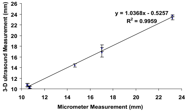
Fig. 10. Correlation between the dimensions measured using the micrometer and the 3D ultrasound system.
