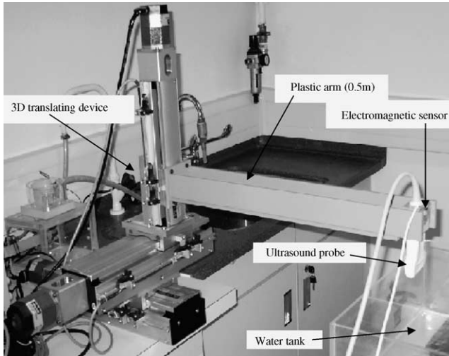
Fig. 3. The 3D translating device used for temporal calibration.
