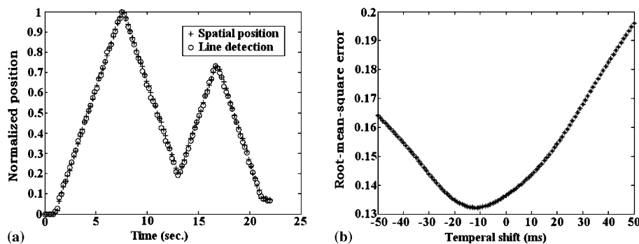
Fig. 4. Temporal calibration results. (a) The position data sets detected by the electromagnetic device and the ultrasound system at the sampling rate of 21 Hz, (b) the root-mean-square errors between the two data sets. The horizontal axis in (a) denotes the measurement time and that in (b) denotes the time delay between the two measurements.
