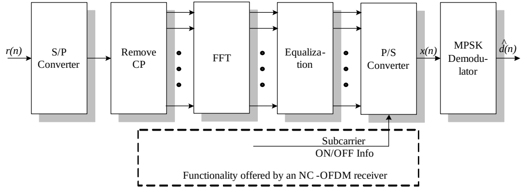
(b) A general OFDM-based receiver
