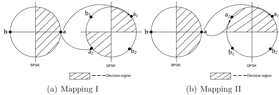
Figure 4.11. Two ways of mapping symbols from BPSK constellation to QPSK
