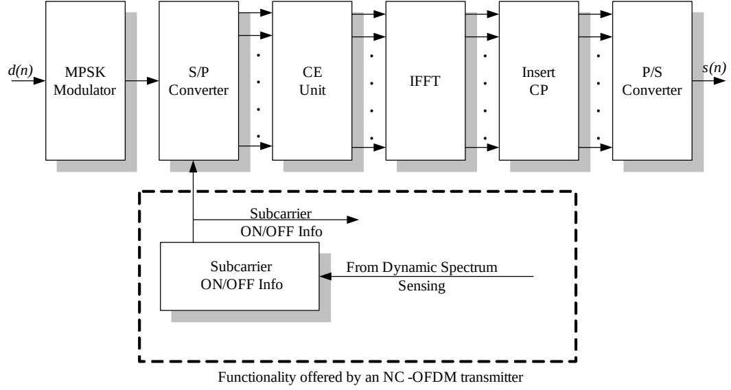
(a) An OFDM-based transmitter employing the CE technique
